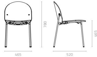
Bobby chair W465 x D520 x H780 x SH465mm Packing: 0.221m 3 , 1pc/ctn
