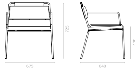
Rope lounge chair W675 x D640 x H725 x SH410mm Packing: 0.350m 3 , 1pcs/ctn
