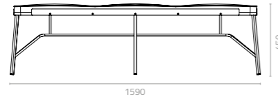
Album bench W1590 x D460 x H450mm Packing: 0.381m 3 , 1pc/ctn
