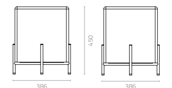
Zora square stool W386 x D386 x H450mm Packing: 0.083m 3 , 1pc/ctn
