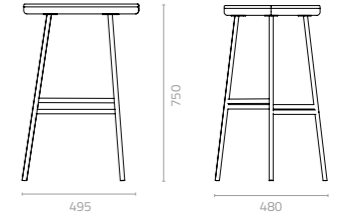
Toru barstool W495 x D480 x H750mm Packing: 0.209m 3 , 1pc/ctn
