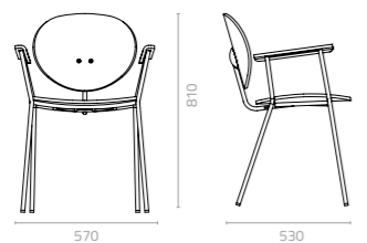
Ovni arm chair W570 x D530 x H810 x SH460mm Packing: 0.270m 3 , 1pc/ctn
