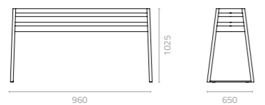
Skyler bar table (frame) W960 x D650 x H1025mm Packing: 0.300m 3 , 1set/2ctns
