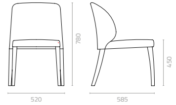
Blow chair W520 x D585 x H780 x SH450mm Packing: 0.470m 3 , 2pcs/ctn Stackable
