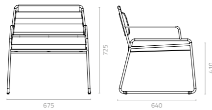
Rope lounge with sled frame W675 x D640 x H725 x SH410mm Packing: 0.350m 3 , 1pc/ctn
