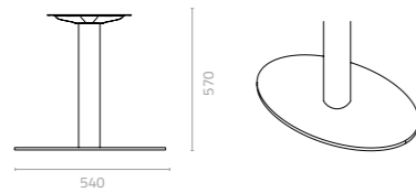
Sharon oval coffee table base W540 x D350 x H570mm Packing: 0.127m 3 , 1set/ctns
