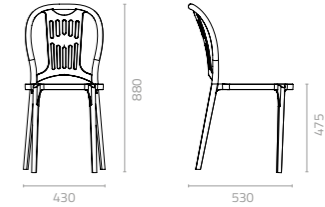
Frank chair W430 x D530 x H880 x SH475mm Packing: 0.402m 3 , 4pcs/ctn Stackable
