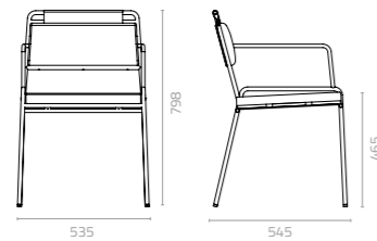
Rope arm chair W535 x D545 x H798 x SH465mm Packing: 0.290m 3 , 1pc/ctn
