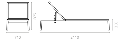
Gradient sunlounger W710 x D2110 x H875 x SH330mm Packing: 1.550m 3 , 2pcs/ctn Stackable
