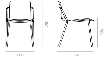
Barra chair W460 x D516 x H790 x SH486mm Packing: 0.212m 3 , 1pcs/ctn
