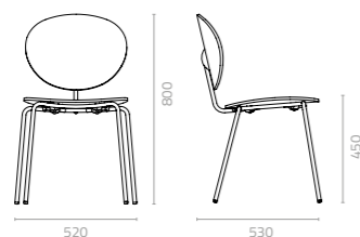
Ovni chair with upholstered seat W520 x D530 x H800 x SH450mm Packing: 0.280m 3 , 4pcs/ctn
