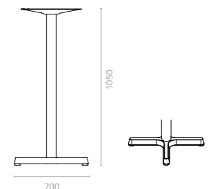
Barkas large bar table base W700 x D505 x H1050 Packing: 0.041m 3 , 2set/3ctns
