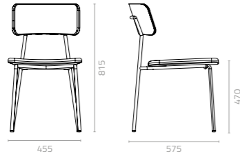
Alumna chair with upholstered seat W455 x D575 x H815 x SH470mm Packing: 0.300m 3 , 2pc/ctn
