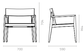
Astras lounge W700 x D590 x H704 x SH394mm Packing: 0.340m 3 , 1pc/ctn
