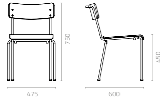
Iota chair W475 x D600 x H750 x SH450mm Packing: 0.310m 3 , 4pcs/ctn Stackable
