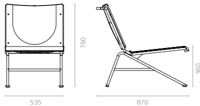
Iota lounge chair W535 x D870 x H760 x SH360 Packing: 0.490m 3 , 2pcs/ctn
