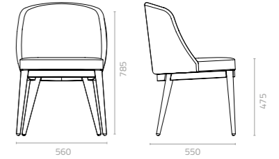
Buona chair W560 x D550 x H785 x SH475mm Packing: 0.270m 3 , 1pc/ctn
