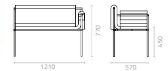
Cirocco booth seating W1210 x D570 x H770 x SH450mm Packing: 0.600m 3 , 1pc/stack
