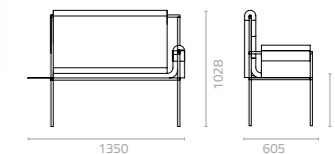
Cirocco high backrest booth seating with side table W1350 x D605 x H1028 x SH450mm Packing: 0.930m 3 , 1pc/stack
