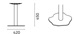
Sharon organic coffee table base W420x D420 x H450mm Packing: 0.464m 3 , 1pcs/1ctn Maximum table top sizes: 800
