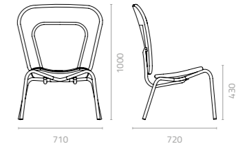
Big Leaf chair W710 x D720 x H1000 x SH430mm Packing: 0.660m 3 , 2pcs/ctn
