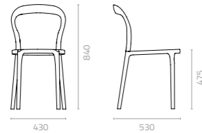
Melrose chair with artwood seat W430 x D530 x H840 x SH475mm Packing: 0.288m 3 , 4pcs/ctn Stackable
