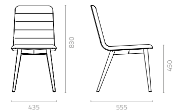
Hook chair W435 x D555 x H830 x SH450mm Packing: 0.340m 3 , 2pcs/ctn
