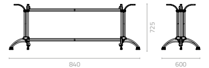
Margherita table base H W840 x D600 x H725mm Packing: 0.225m 3 , 1pc/ctn
