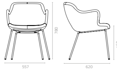
Bebo arm chair-4 legged slim W557 x D620 x H780 x SH460mm Packing: 0.310m 3 , 1pc/ctn
