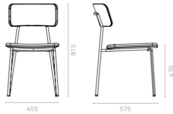
Alumna chair with upholstered seat W455 x D575 x H815 x SH470mm Packing: 0.300m 3 , 2pc/ctn
