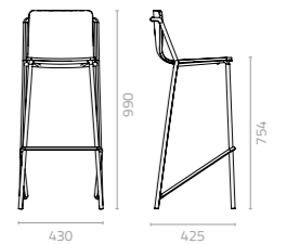
Barra barstool W430 x D425 x H990 x SH754mm Packing: 0.220m 3 , 1pc/ctn
