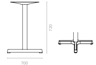
Barkas large table base W700 x D505 x H720 Packing: 0.040m 3 , 2set/3ctns
