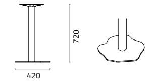
Sharon organic dining table base W420 x D420 x H720mm Packing: 0.288m 3 , 1pcs/ctn Maximum table top sizes: 800
