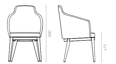
Buona high back chair W570 x D570 x H880 x SH475mm Packing: 0.310m 3 , 1pc/ctn
