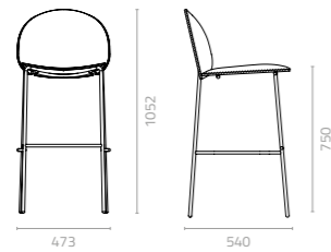
Bobby barstool W473 x D540 x H1052 x SH750mm Packing: 0.310m 3 , 1pc/ctn
