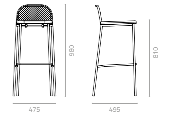
Mogen barstool W475 x D495 x H980 x SH810mm Packing: 0.270m 3 , 1pc/ctn
