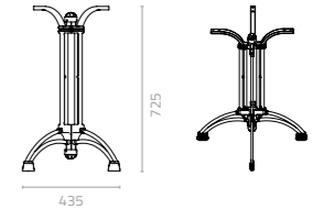
Margherita table base W435 x D435 x H725mm Packing: 0.151m 3 , 1pc/ctn
