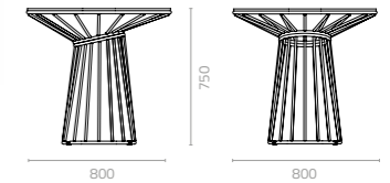
Wins dining table W800 x D800 x H750mm Packing: 0.500m 3 , 1pc/stack
