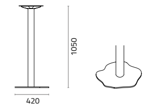
Sharon organic bar table base W420x D420 x H1050mm Packing: 0.464m 3 , 1pcs/1ctn Maximum table top sizes: 800
