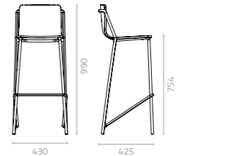
Barra barstool W430 x D425 x H990 x SH754mm Packing: 0.220m 3 , 1pc/ctn
