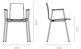
Zeat arm chair - wooden arm W565 x D505 x H810 x SH455mm Packing: 0.393m 3 , 4pcs/ctn Stackable
