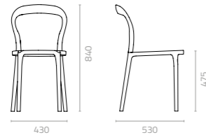
Melrose chair with textile seat W430 x D530 x H840 x SH475mm Packing: 0.290m 3 , 4pcs/ctn Stackable
