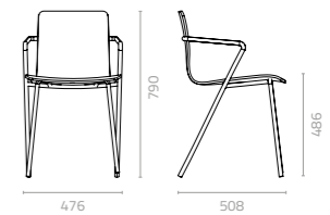
Barra arm chair W476 x D508 x H790 x SH486mm Packing: 0.270m 3 , 1pc/ctn
