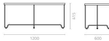
Matrix rectangular coffee table W1200 x D600 x H415 Packing: 0.406m 3 , 2stacks/set
