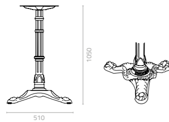
Cappuccino 3 bar table base W510 x D450 x H1050 Packing: 0.275m 3 , 1pc/ctn
