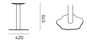
Sharon organic side table base W420x D420 x H570mm Packing: 0.464m 3 , 1pcs/1ctn Maximum table top sizes: 800
