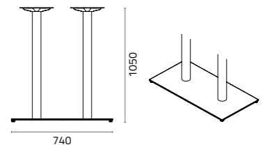
Sharon rectangular 2 poles bar table base W740x D485 x H1050mm Packing: 0.464m 3 , 1pcs/1ctn Maximum table top sizes: 1200
