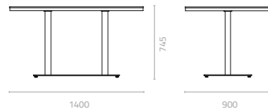
Gradient double shaft dining table W1400 x D900 x H745mm Packing: 0.120m 3 , 3ctns/set
