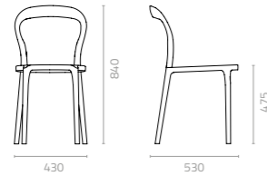
Melrose chair with PP seat W430 x D530 x H840 x SH475mm Packing: 0.288m 3 , 4pcs/ctn Stackable
