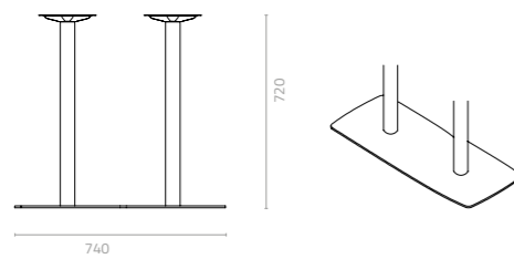
Sharon convex 2 pole table base W740 x D485 x H720mm Packing: 0.094m 3 , 1pc/ctn
