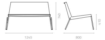
Gradient 2-seater lounge chair W1245 x D800 x H740 x SH410mm Packing: 0.980m 3 , 2pcs/ctn Stackable
