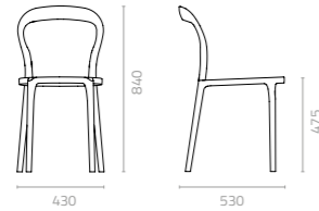
Melrose chair with wicker seat W430 x D530 x H840 x SH475mm Packing: 0.290m 3 , 4pcs/ctn Stackable
