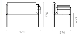
Cirocco booth seating with cushion W1210 x D570 x H770 x SH450mm Packing: 0.600m 3 , 1pc/ctn
