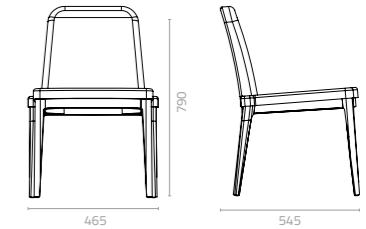
Eli chair W465 x D545 x H790 x SH450mm Packing: 0.270m 3 , 1pc/ctn
