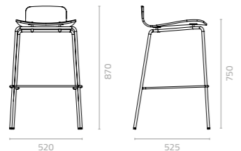
Zeat barstool W520 x D525 x H870 x SH750mm Packing: 0.393m 3 , 4pcs/ctn Stackable
