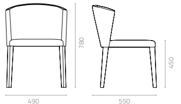
Cady chair W490 x D550 x H780 x SH450mm Packing: 0.460m 3 , 2pcs/ctn Stackable
